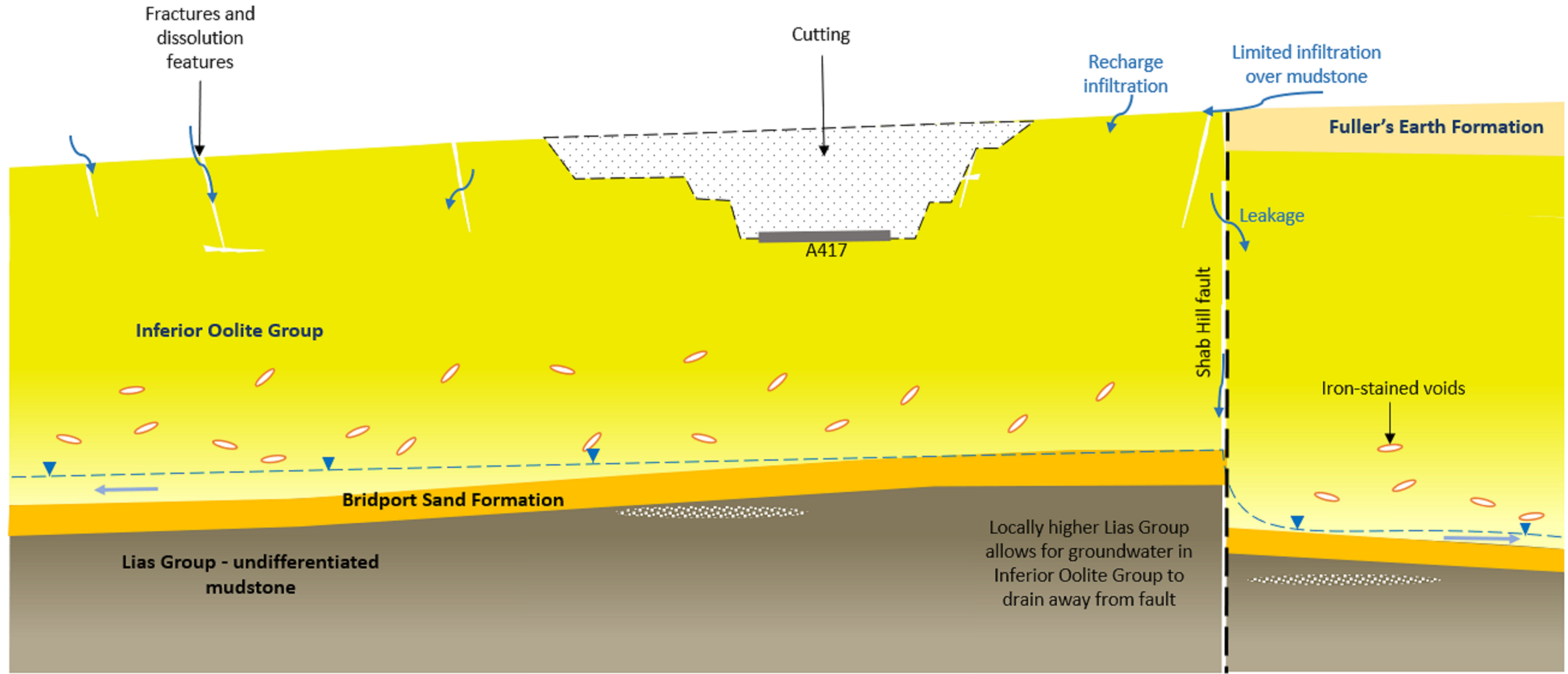
SECTION F - F' CH. 2+750 AIR BALLOON CUT
